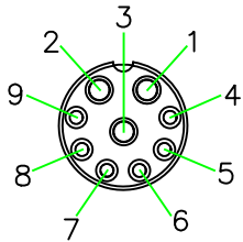
PIN ASSIGNMENT FRONT VIEW (前視圖)
