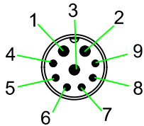
PIN ASSIGNMENT FRONT VIEW (前視圖)
