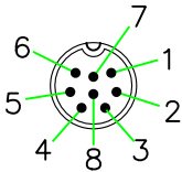
PIN ASSIGNMENT FRONT VIEW (前視圖)
