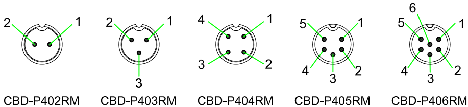
PIN ASSIGNMENT FRONT VIEW (前視圖)
