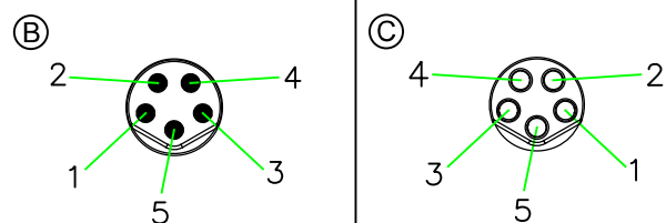
PIN ASSIGNMENT FRONT VIEW (前視圖)
