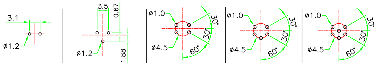
PCB LAYOUT
