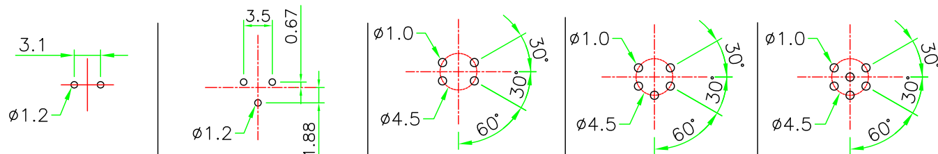
PCB LAYOUT
