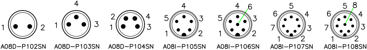
PIN ASSIGNMENT FRONT VIEW (前視圖) △1
