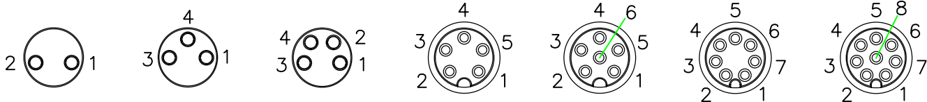
PIN ASSIGNMENT FRONT VIEW (前視圖)
