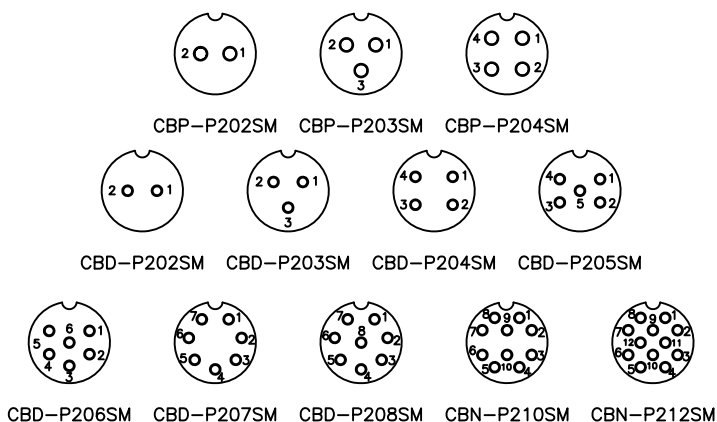
PIN ASSIGNMENT FRONT VIEW
