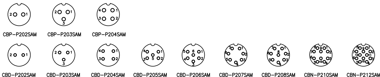
PIN ASSIGNMENT FRONT VIEW (前視圖)
