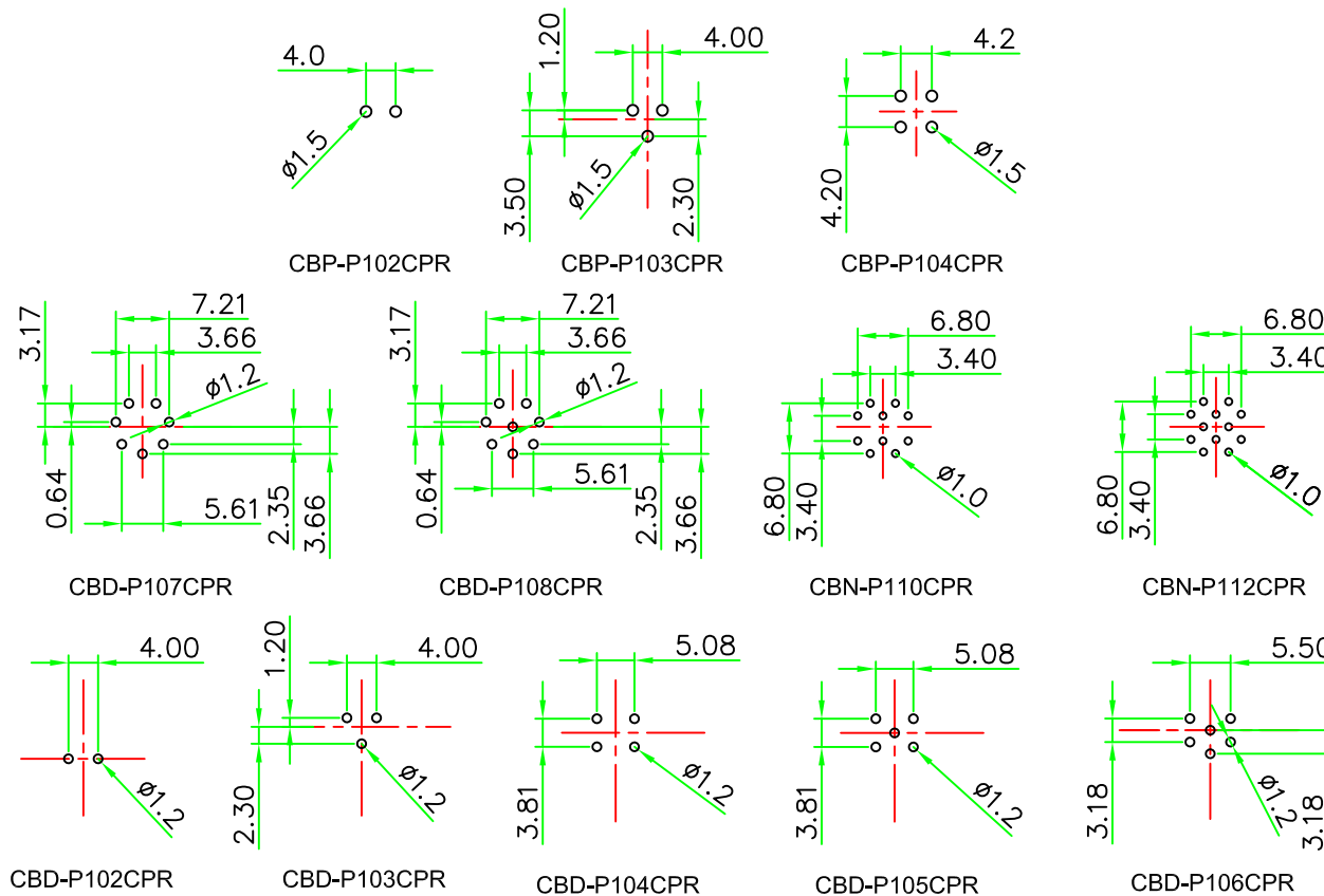
PCB LAYOUT
