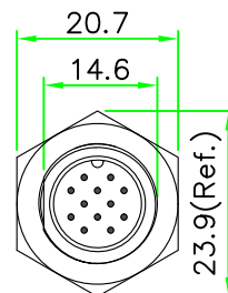
FRONT VIEW (前視圖)
