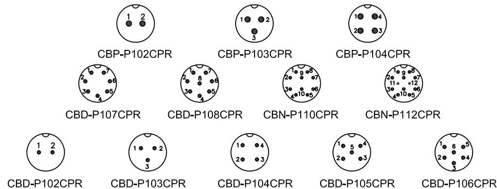
PIN ASSIGNMENT FRONT VIEW (前視圖)
