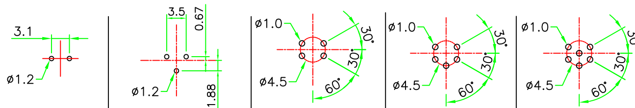
PCB LAYOUT
